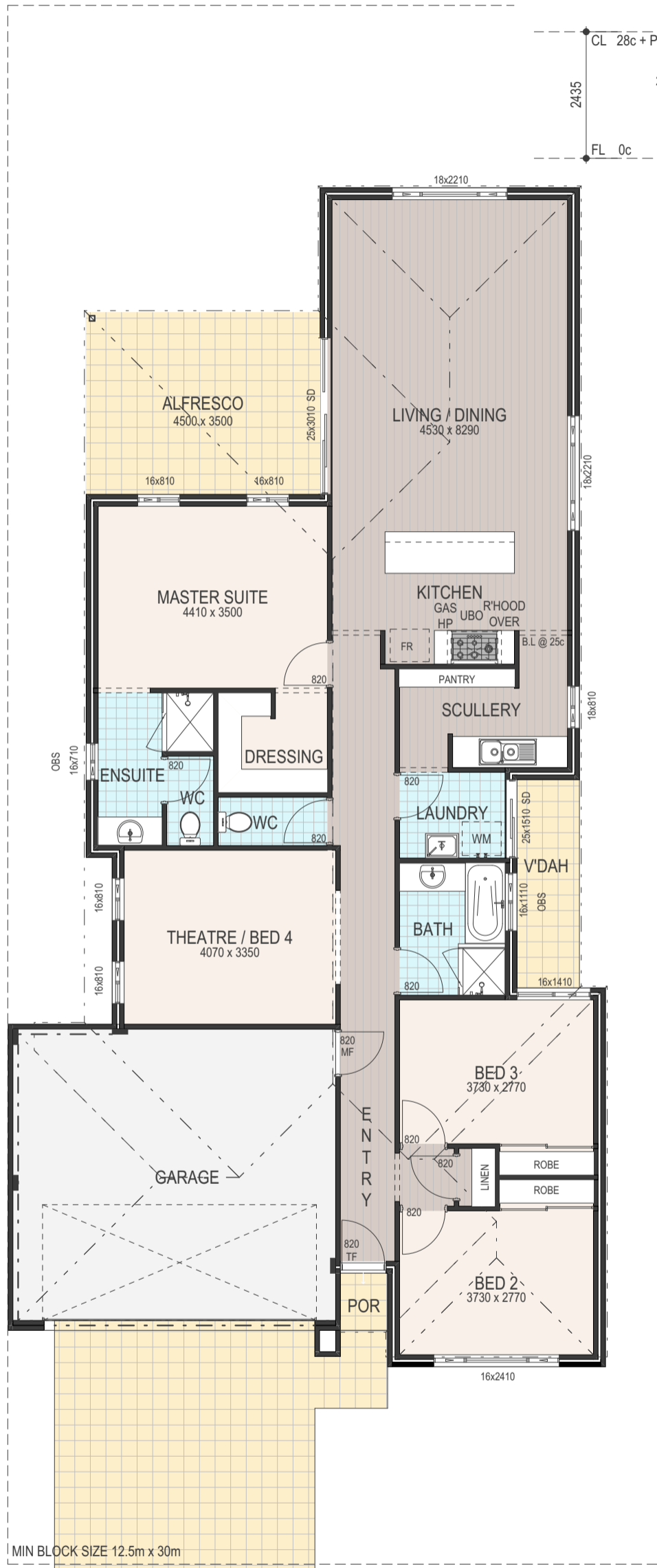
FLOOR PLAN 1:100
